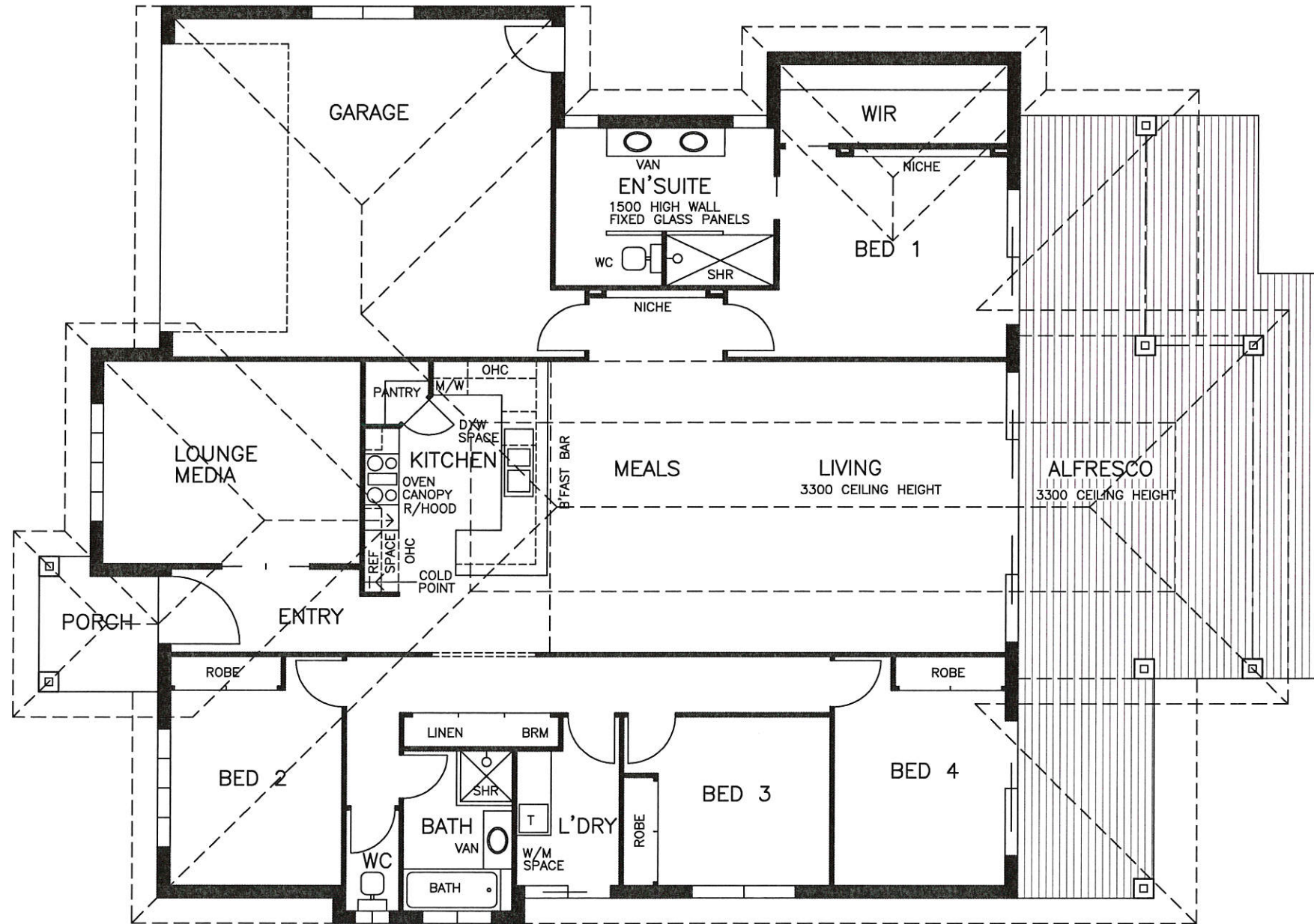
FLOOR PLAN
